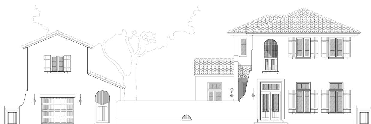
Floor Plan / Site Plan & Front Elevation, Sideyard House – New Construction Courtney Residence, Coral Gables FL. 2016-2017 (Under Construction)
