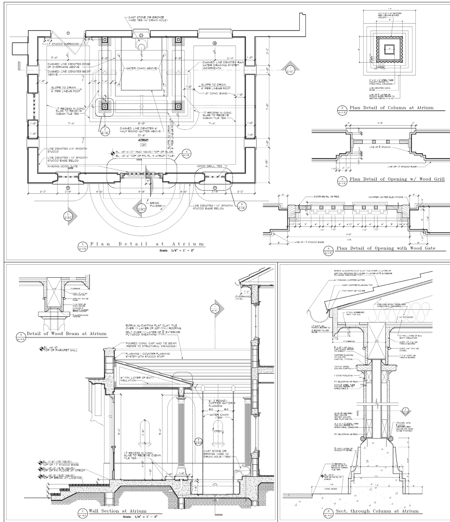
Detail Drawings - New Construction Janzon Residence, Baypoint, Miami, FL. Winner of Addison Mizner Medal by the Institute of Classical Architecture, 2013
